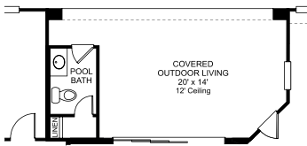
OPTIONAL 12' x 8' SLIDING GLASS DOOR W/ POOL BATH
