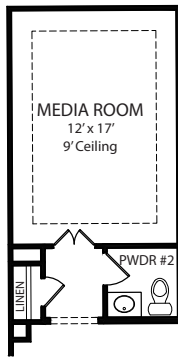
OPTIONAL MEDIA ROOM W/ POWDER
